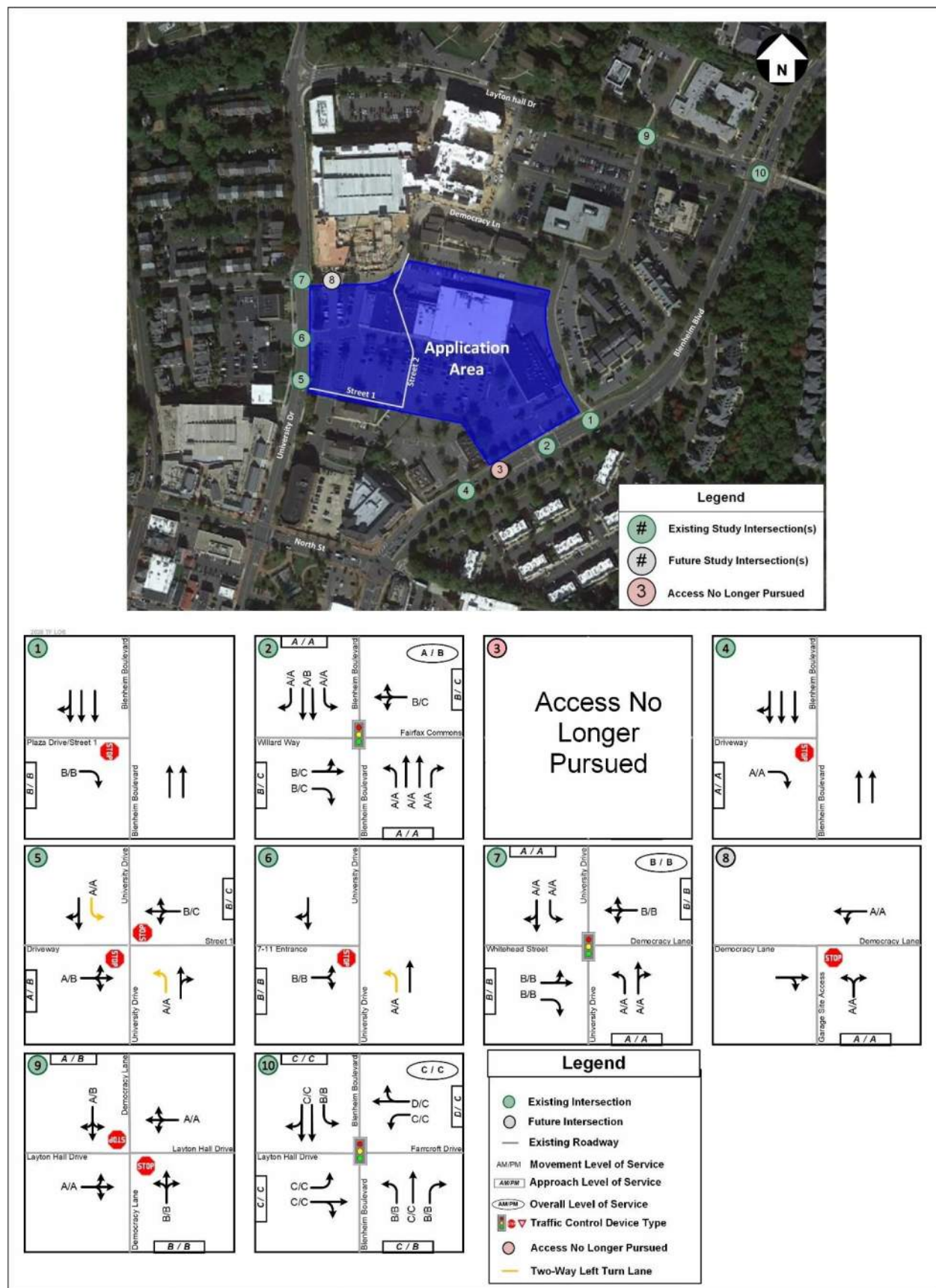
Figure 34: 2028 Future with Development Level of Service Results (Full-Build)
