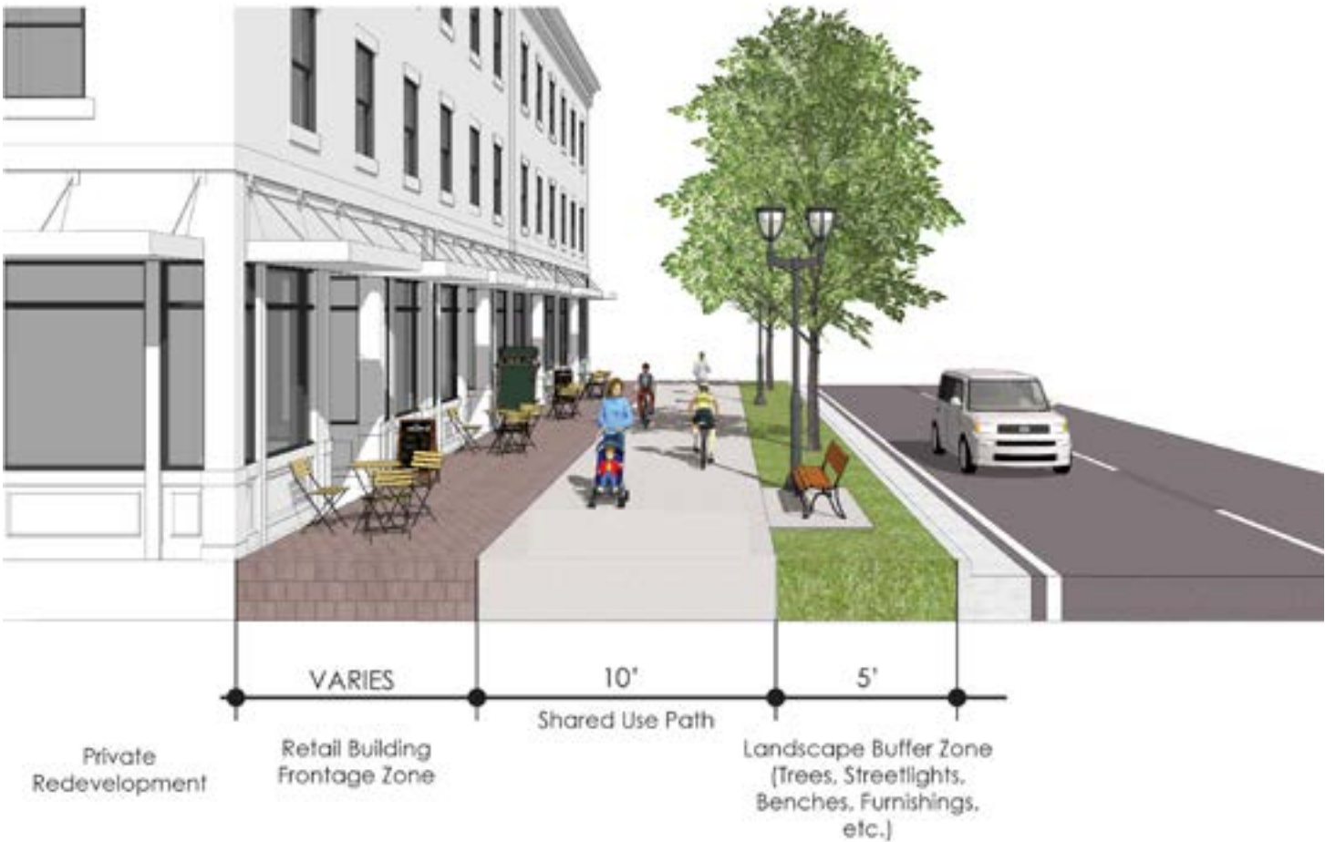
TYPICAL SHARED USE PATH - RETAIL SHOWN REFER TO FRONTAGE DIAGRAMS (pg. 34)
