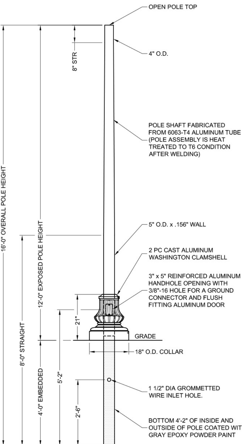
LIGHT POST - VALMONT Embedded Aluminum Pole
