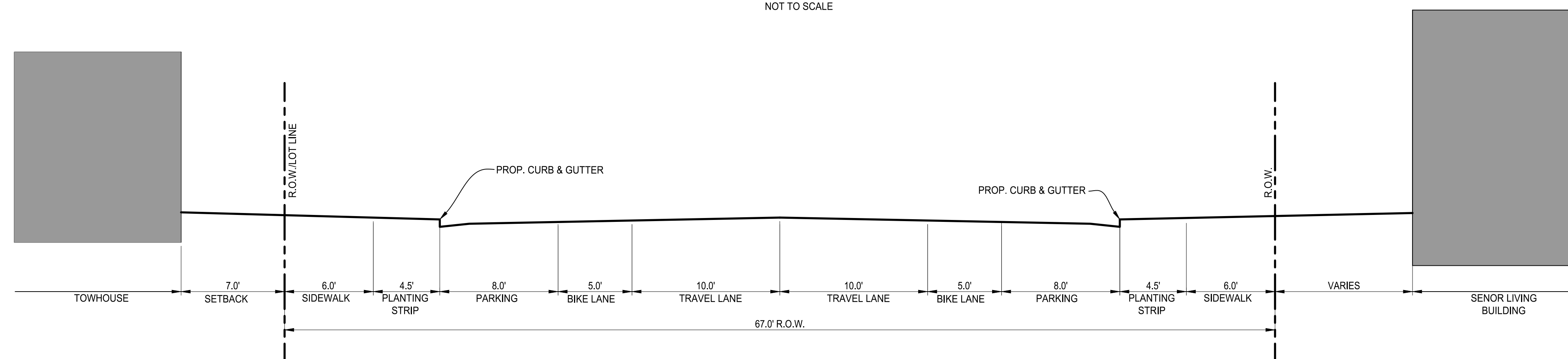
FARR AVENUE TYPICAL SECTION NOT TO SCALE
