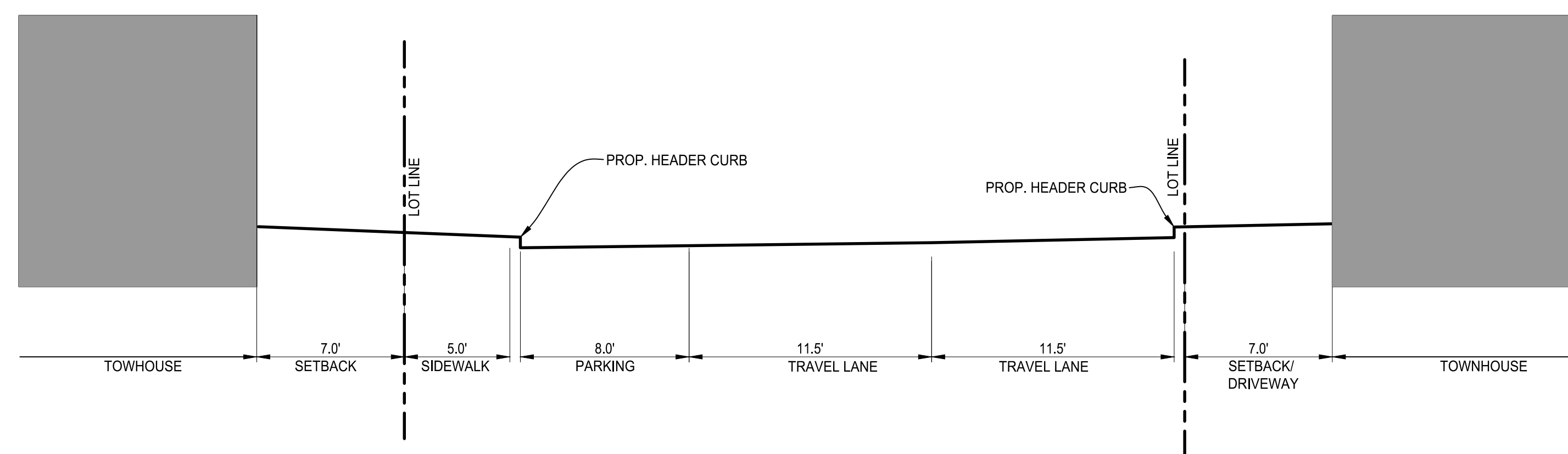
PRIVATE STREET TYPICAL SECTION NOT TO SCALE
