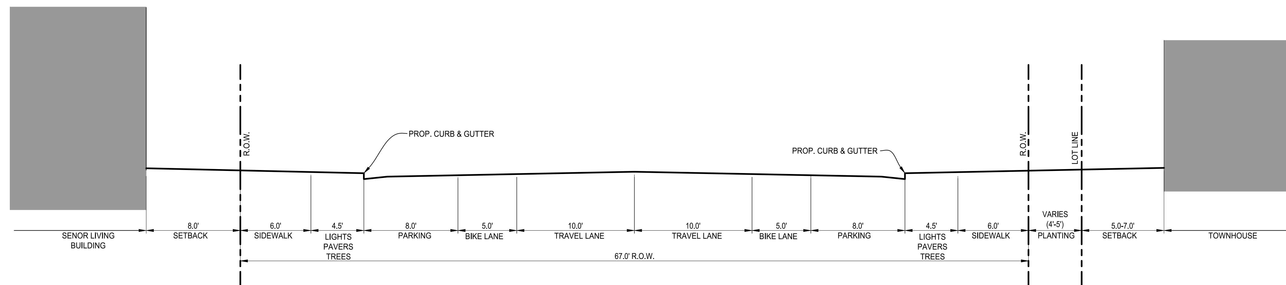
ORCHARD STREET TYPICAL SECTION NOT TO SCALE
